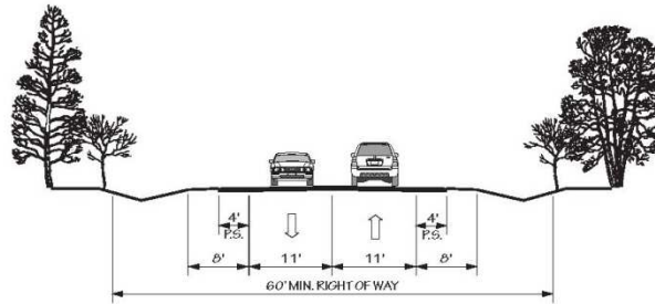
TYPICAL SECTION No. 2B 2 LANE UNDIVIDED WITH PAVED SHOULDERS
